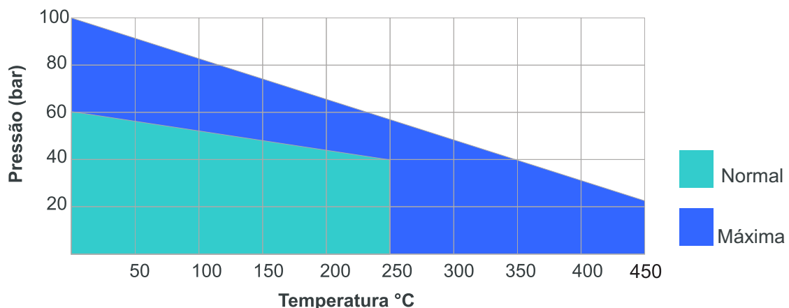
Diagrama P x T
